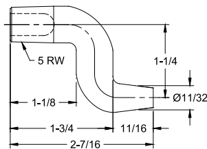
16-38666 RWMA CLASS 2 COLD FORMED*
