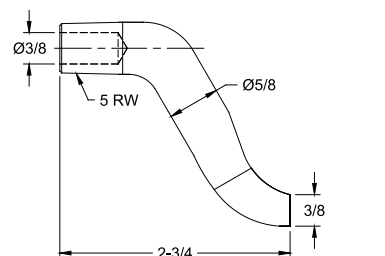
16-38353 RWMA CLASS 2 COLD FORMED*
