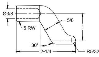
16-3836 RWMA CLASS 2 CASTING
