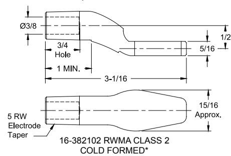
Bent Dimensions for Reference Only
