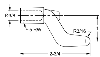
16-3838 RWMA CLASS 2 CASTING
