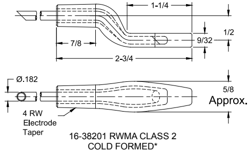
Bent Dimensions for Reference Only
