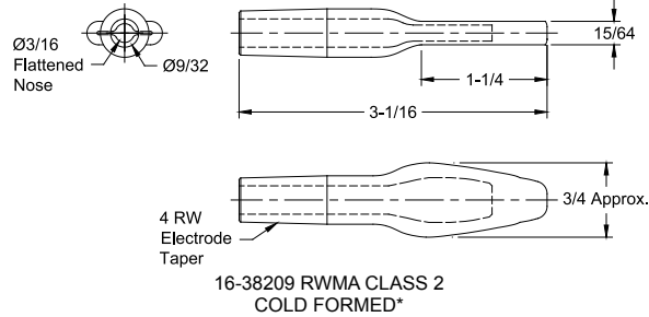
Bent Dimensions for Reference Only
