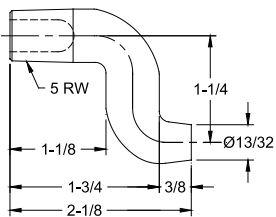
16-38661 RWMA CLASS 2 COLD FORMED*
