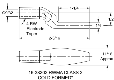
Bent Dimensions for Reference Only
