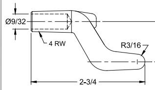
16-3837 RWMA CLASS 2 CASTING
