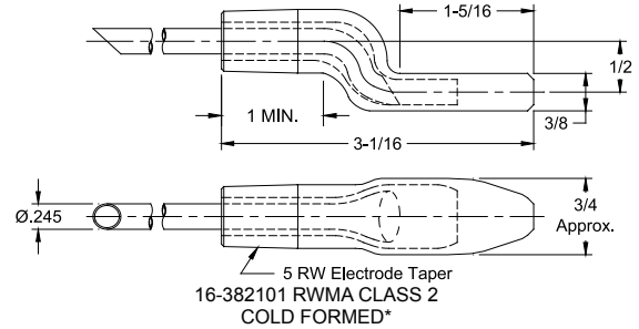
Bent Dimensions for Reference Only
